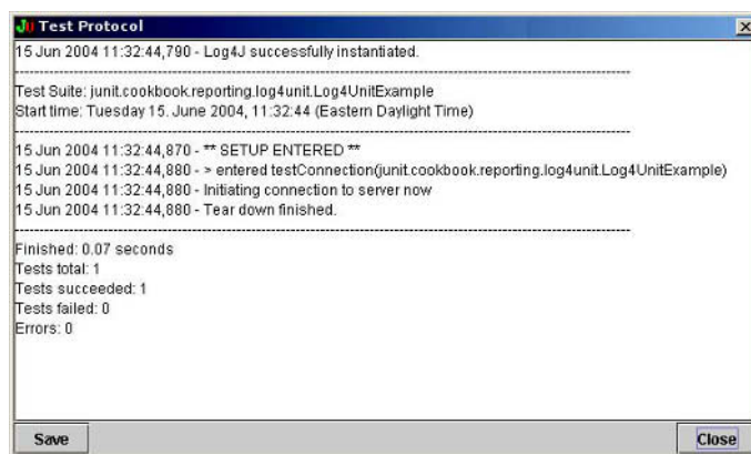
Figure 7.2 The Log4Unit Test Protocol dialog box, showing log statements and test summary information
